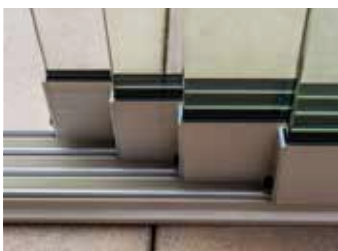
Floor frame
